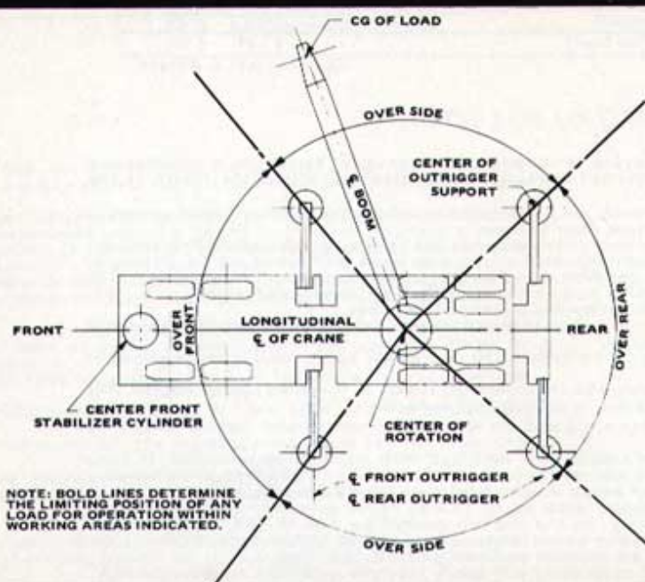
LIFTING AREA DIAGRAM
