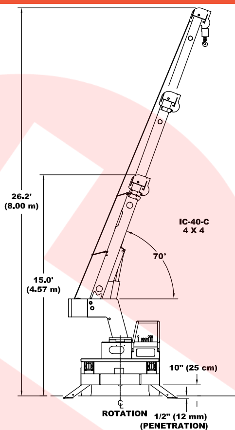
IC-40-2C Chart
